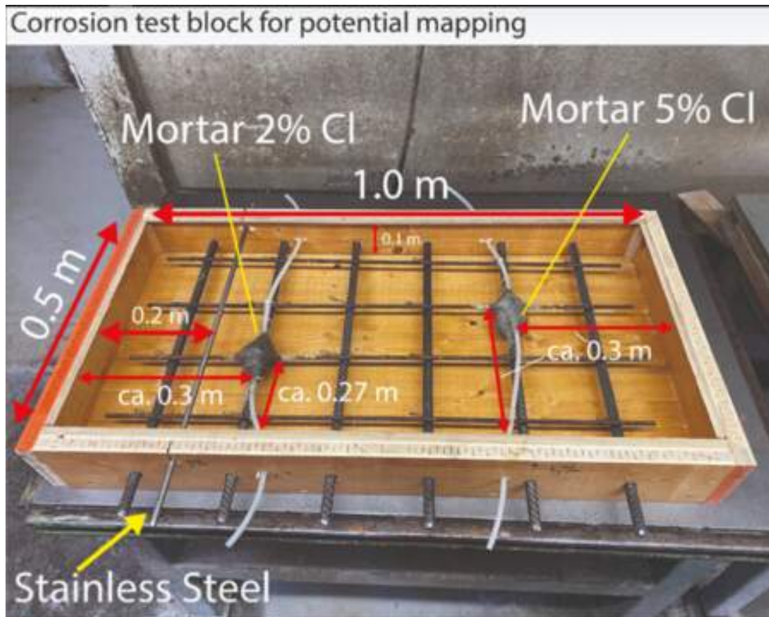
Note: only the lowest left anode (2% Cl) was activated in this test.
